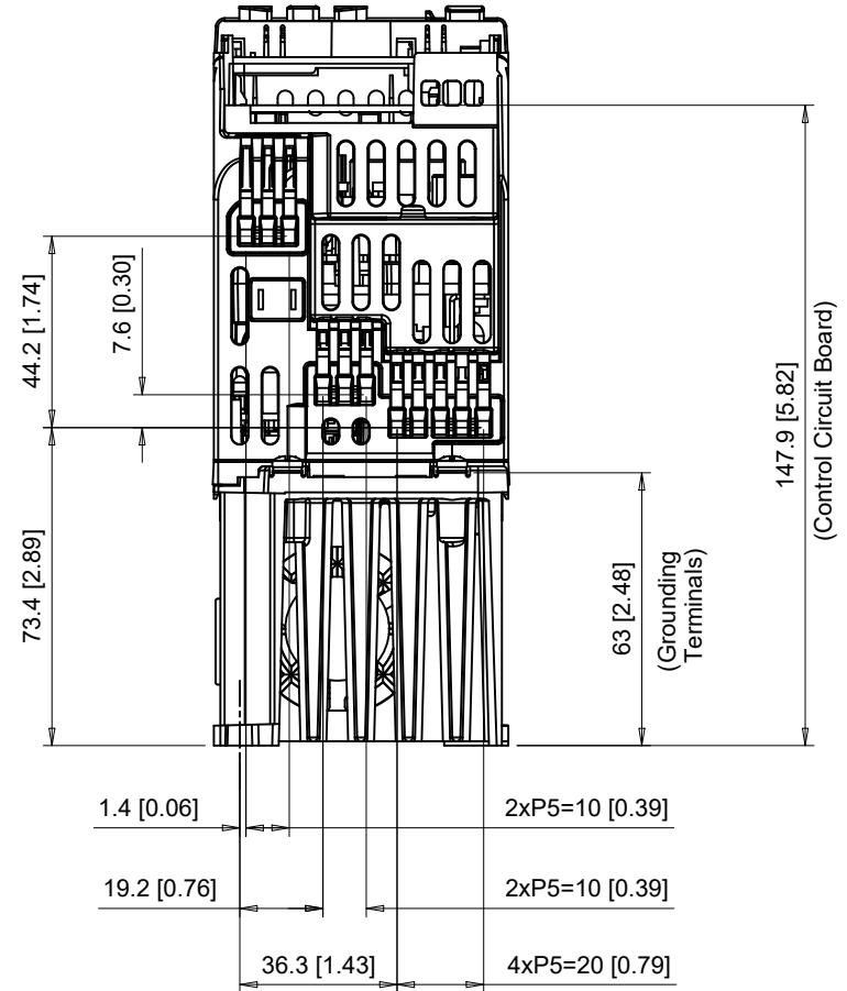
BOTTOM VIEW
