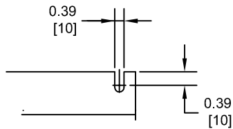
Mounting hole specifications
