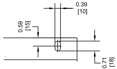
Mounting hole specifications
