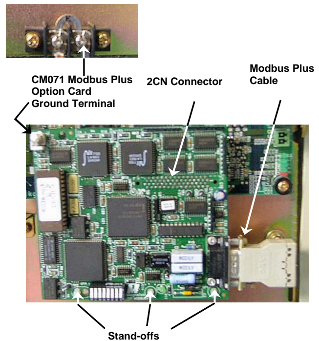
Attaching the CM071 Modbus Plus Option on a G5HHP master control board.
