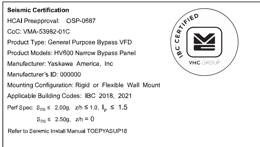
Figure 2.2 Seismic Certification Label Example for Bypasses and Configured Packages
